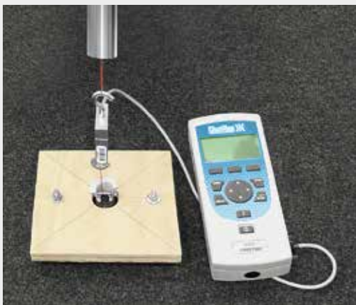
Testing of fixing element strength
